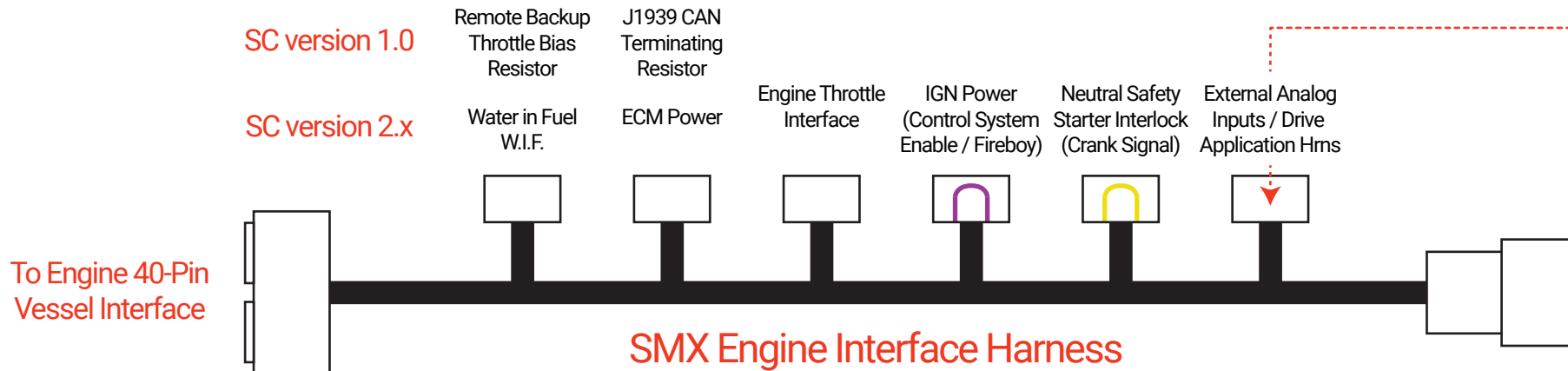
SMX Drive Application Harness
