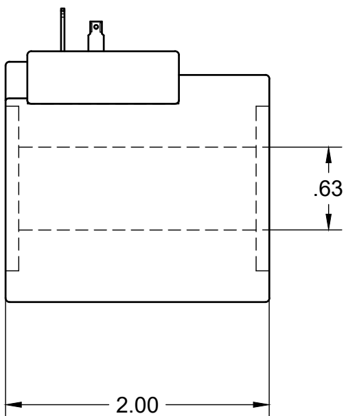
ZF EB30 SHIFT SOLENOID COIL BASIC DIMENSIONS
