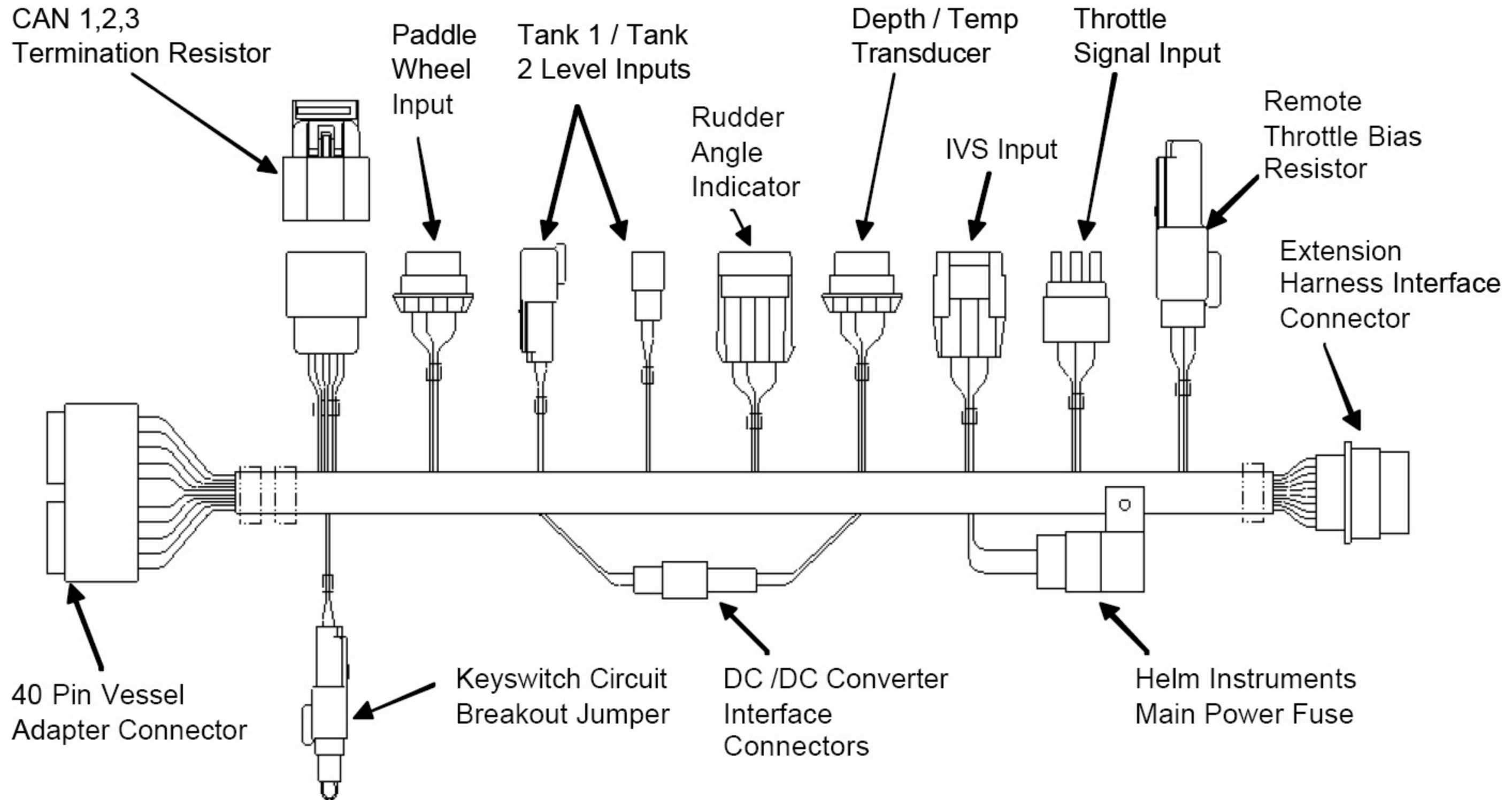
FIGURE 33: VESSEL ADAPTER HARNESS
