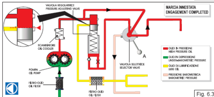
Typical ZF Hydraulic Circuit and Power Flow Diagrams
