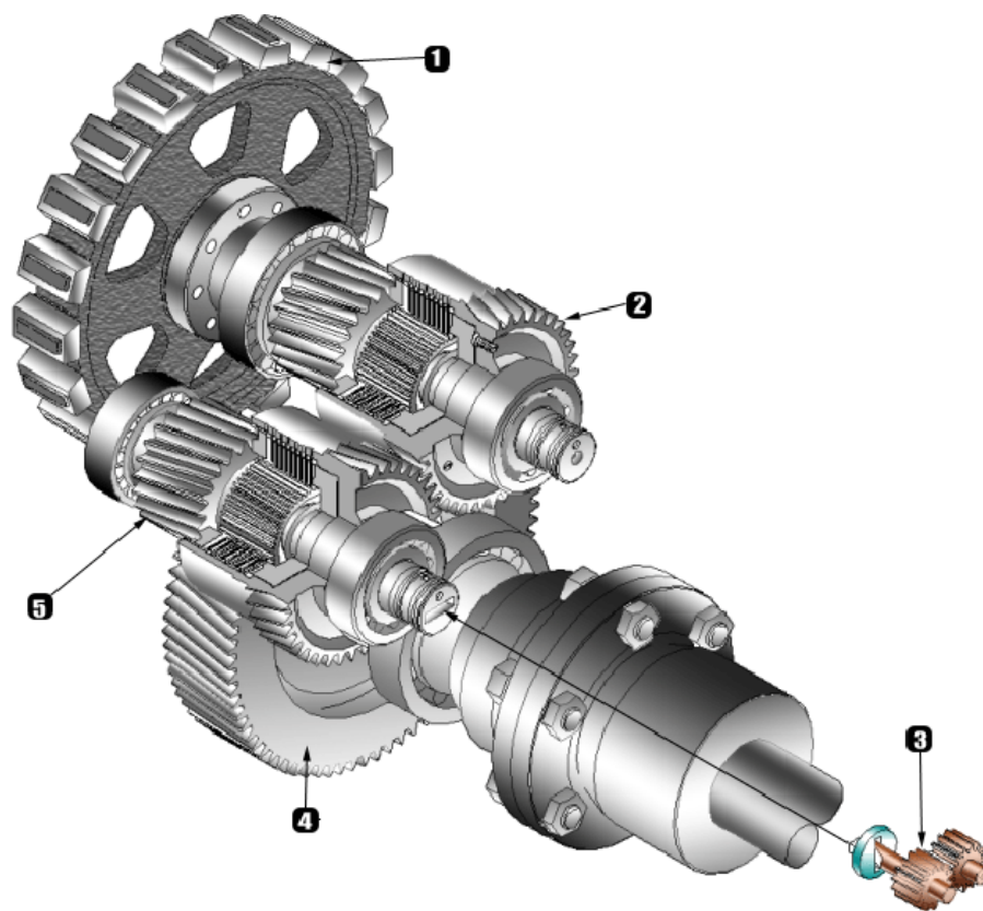
Typical 3-Shaft Full Reversing Transmission
